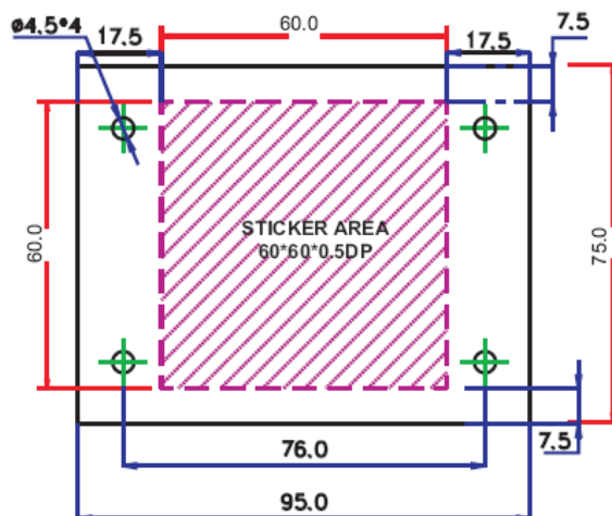
Mounting Detail
